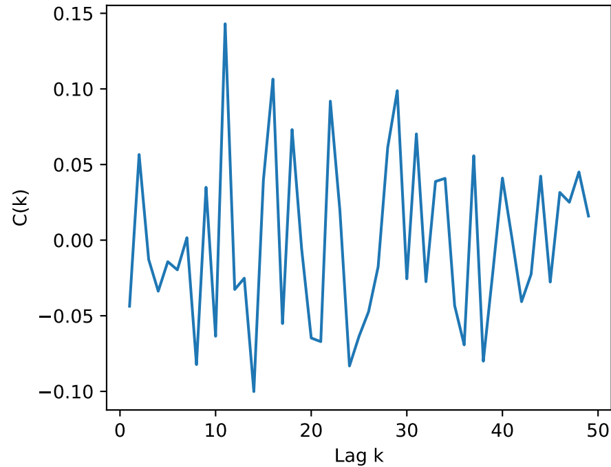
HOMO Autocorrelation
