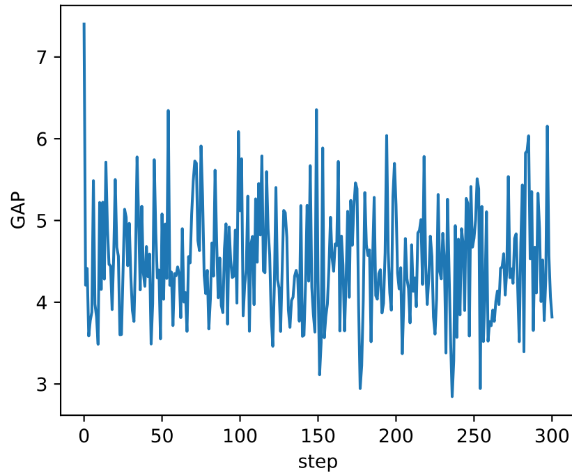
GAP - evolution
