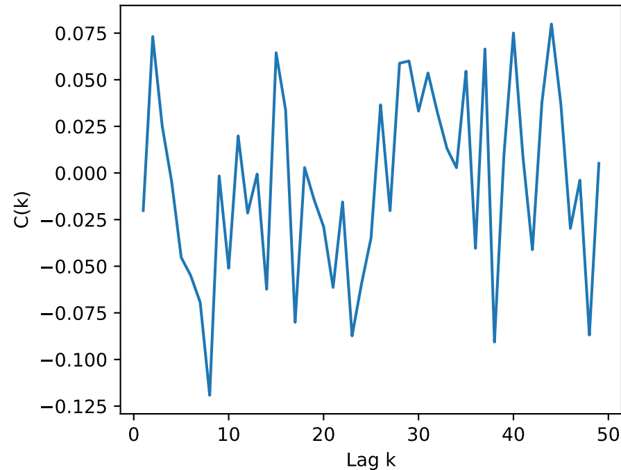
LUMO Autocorrelation
