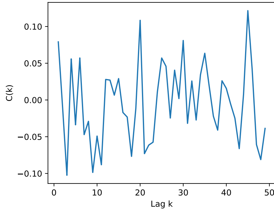
GAP Autocorrelation
